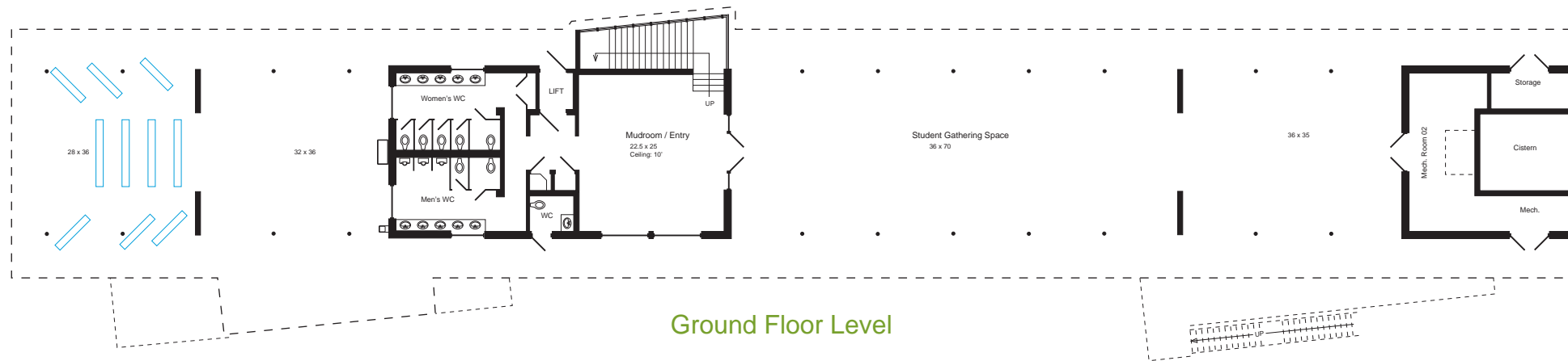
Environmental Learning Centre Lower Level Layout
